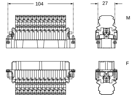
contacts side (front view)
