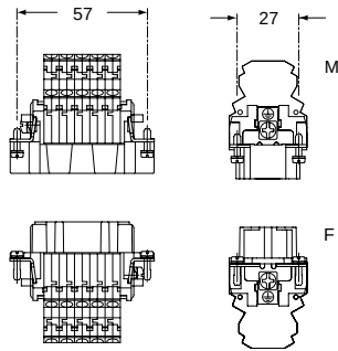
contacts side (front view)
