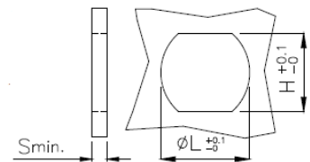
PANEL HOLE
