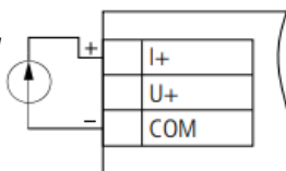
Stromsignal / current sensor wiring
