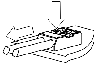
Fig. 5.3 Disconnecting the wire
