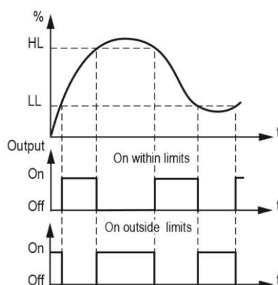
Fig. 6.2 Output control
